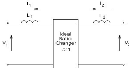
Figure 6-3 - 'Ideal' Transformer Equivalent Circuit
