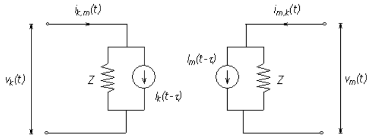
Figure 8-29 – EMTDC Distributed Branch Interface (Single-Phase)
