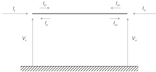
Figure 8-38 – Voltages and Currents in an N -Conductor Transmission Line
