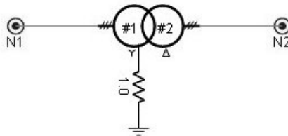
Figure 2-6 – Simple 3-Phase, 2-Winding Transformer Module Canvas
