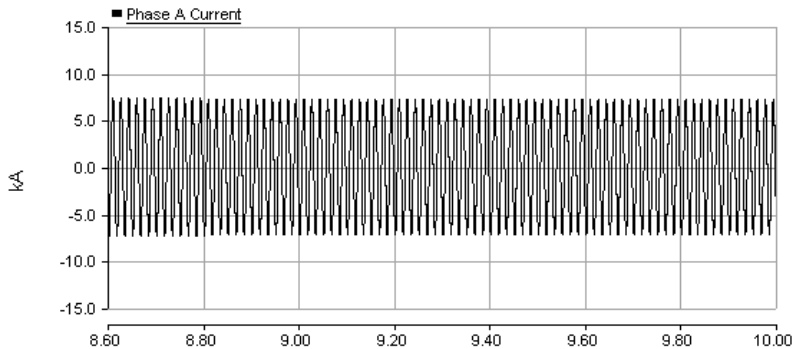
Figure 7-T7 - Steady-State Fault Current
