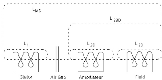
Figure 7-3 - Flux Paths Associated with Various d-axis Inductances
