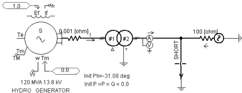
Figure 7-T1 - Short-Circuit Test Circuit in PSCAD
