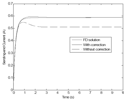
Figure 8-24 – Time domain Results for a Short Circuit Condition
