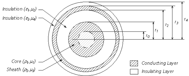
Figure 8-6 - Cross-Section of a 2-Conducting Layer SC Cable
