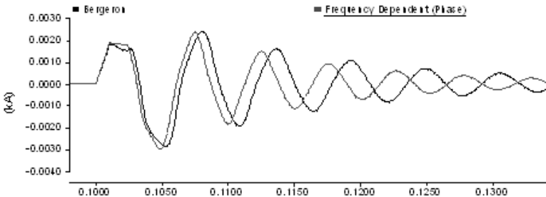
Figure 8-35 – Bergeron Response with High Frequency Attenuation
