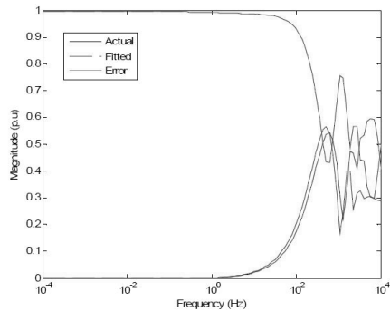
Figure 8-23 – Frequency Response Plots for the Elements of the First Column of the Propagation Matrix
